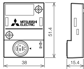
FX5-422-BD-GOT
